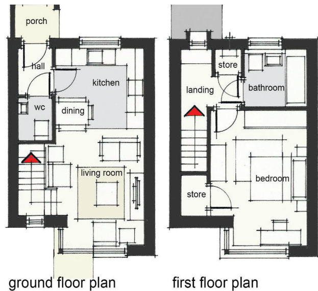
Typical floor plan - 58 SQM
